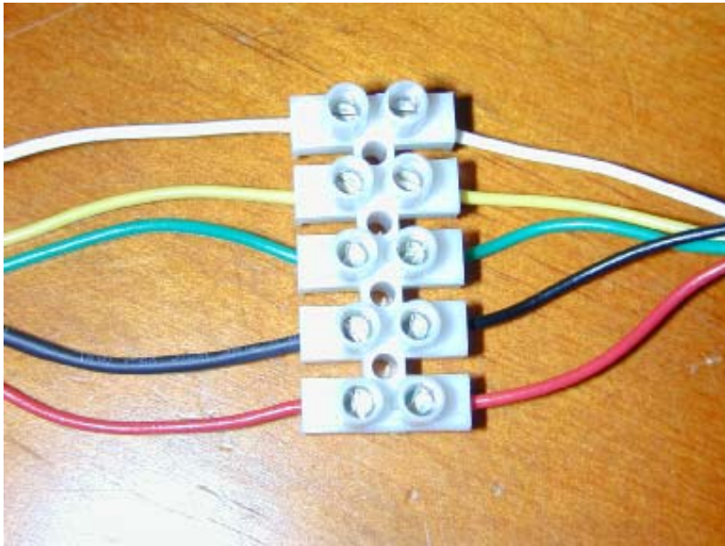
Figure 6 - Connecting to the CruzPro WS110 Wind Display
